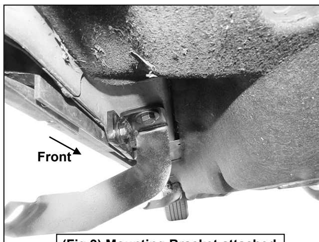
(Fig 9) Mounting Bracket attached to the Driver/Left rear location
